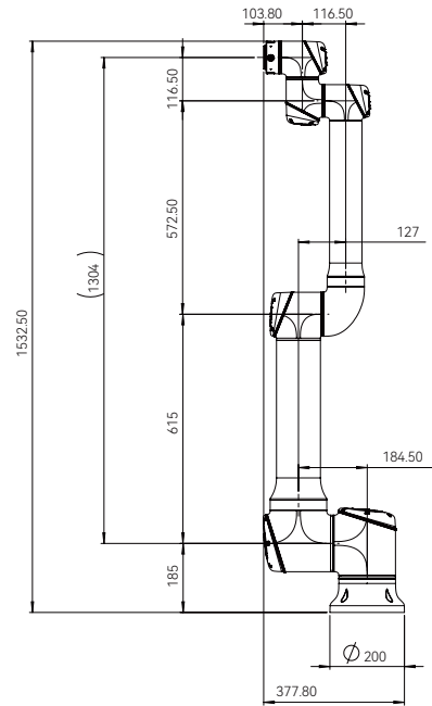
EC612 external dimensional drawing
