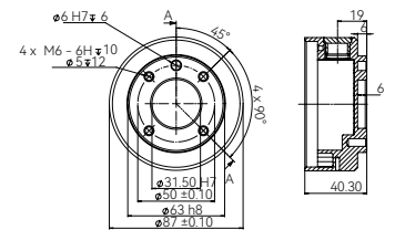
EC612 end flange
