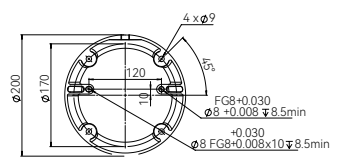
EC612 base top view
